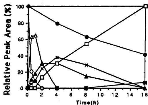
Figure 5. Metabolism of HP 2 DDC (2) in the presence of rat brain cytosol: (○) HP 2 DDC (2); (Δ) O-P, N-HPDDC; (▲) N-HPDDC; (×) N-PDDC; (□) DDC.
