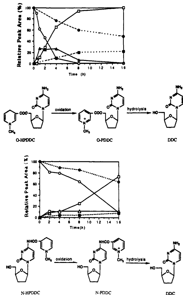
Figure 4. Metabolic transformations of O-HPDDC (3) and N-HPDDC (4) in the presence of rat brain cytosolic extract. Top panel: conversion of O-HPDDC (○) to O-PDDC (Δ) and DDC (□). In the absence of rat cytosol, there was a relatively slow decomposition of O-HPDDC (●), but little DDC (■) was formed. Bottom panel: transformations of N-HPDDC (○) to DDC (□) and N-PDDC (Δ). The decomposition of N-HPDDC under the same conditions but in the absence of rat brain extract (●) gave rise to little DDC (■).
